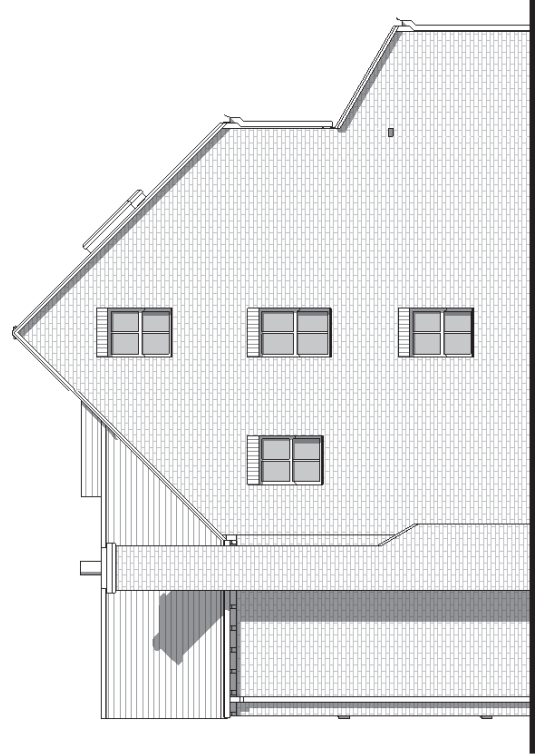
Side Elevation. 1 : 100
